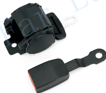
C025 YO.4A通用型紧急锁止自动二点安全带 Universal Type ELR 2-point Seat Belt
