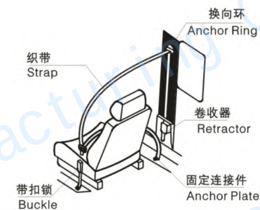
紧急锁止式三点安装图 ELR 3-Point Seat Belt Installation Diagram
