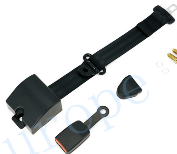
C026 YO.4A欧标型紧急锁止自动二点安全带 European Standard ELR 2-point Seat Belt
